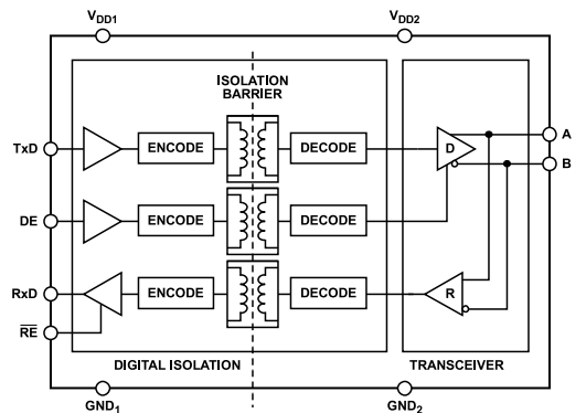
Figure 26. Digital Isolation and Transceiver Sections
