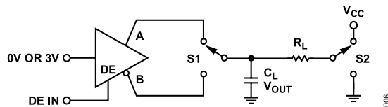
Figure 19. Driver Enable/Disable
