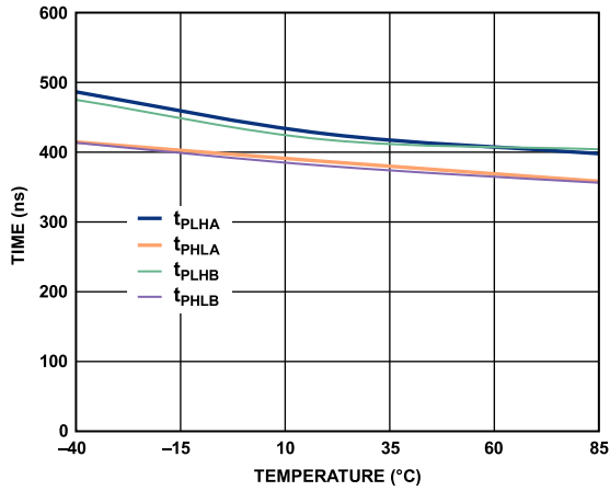
Figure 9. Driver Propagation Delay vs. Temperature
