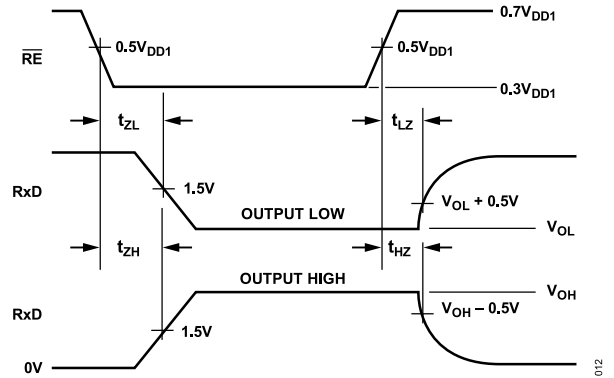
Figure 25. Receiver Enable/Disable Timing
