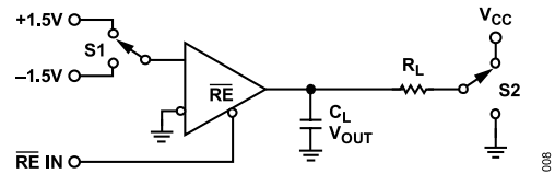
Figure 21. Receiver Enable/Disable
