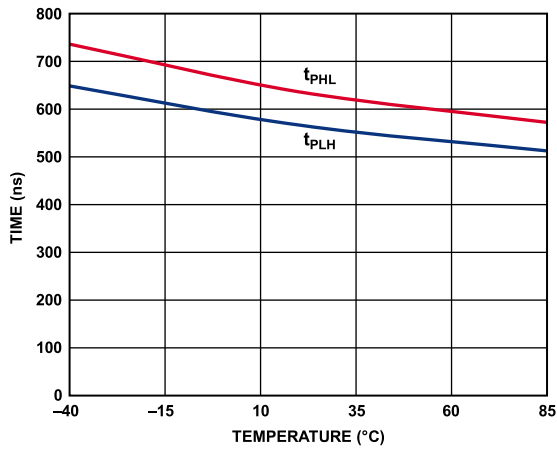
Figure 10. Receiver Propagation Delay vs. Temperature
