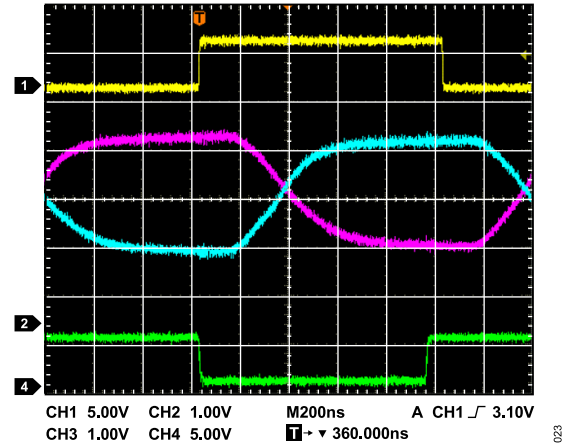
Figure 12. Driver/Receiver Propagation Delay, Low to High
