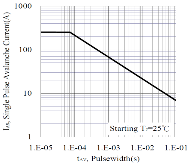
Figure 9: Avalanche Characteristics
