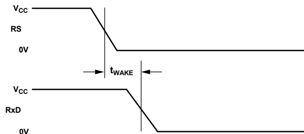
Figure 28. Wake-Up Delay Returning from Standby Mode
