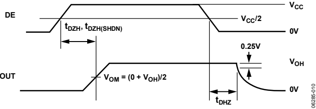
Figure 10. Driver Enable and Disable Times ( t_{DZH} , t_{DZH(SHDN)} )
