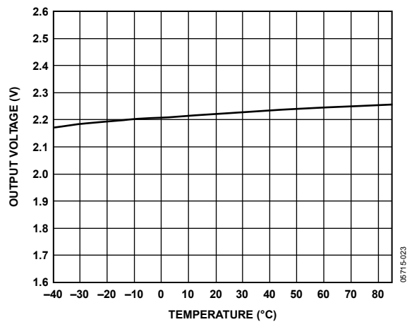
Figure 23. Driver Differential Output Voltage vs. Temperature, R I = 54 Ω
