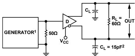
Figure 6. Driver Differential Output Delay and Transition Times
