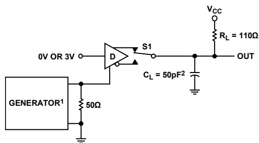
Figure 9. Driver Enable and Disable Times ( t_{PZL} , t_{PSL} , t_{PLZ} )
