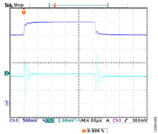
Figure 55. Line Transient Response, 2.5 V to 3 V, I_{LOAD} = 2\text{ A} , Adjustable Version, V_{OUT} = 1.2\text{ V} , CH1 = V_{IN} , CH2 = V_{OUT}
