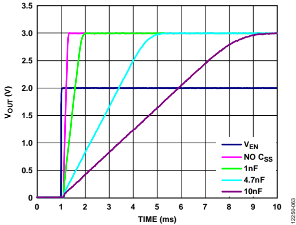
Figure 63. Typical Soft Start Behavior, Different C SS Values
