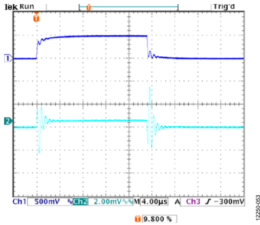
Figure 53. Line Transient Response, 6 V to 6.5 V, I_{LOAD} = 2\text{ A} , V_{OUT} = 5\text{ V} , CH1 = V_{IN} , CH2 = V_{OUT}
