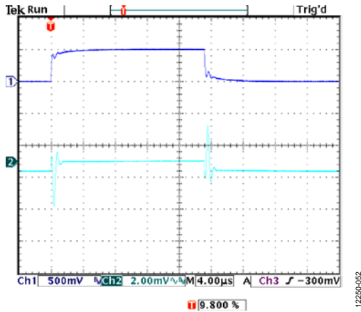
Figure 52. Line Transient Response, 6 V to 6.5 V, I_{LOAD} = 500\text{ mA} , V_{OUT} = 5\text{ V} , CH1 = V_{IN} , CH2 = V_{OUT}
