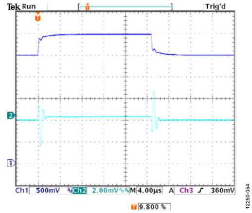
Figure 54. Line Transient Response, 2.5 V to 3 V, I_{LOAD} = 500\text{ mA} , Adjustable Version, V_{OUT} = 1.2\text{ V} , CH1 = V_{IN} , CH2 = V_{OUT}
