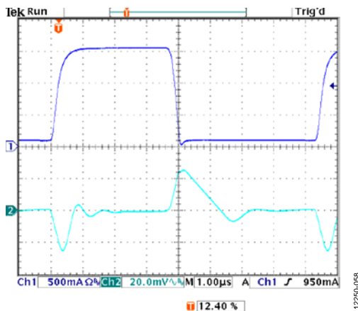
Figure 58. Output Transient Response, V_{OUT} = 5\text{ V} , C_{OUT} = 4.7\ \mu\text{F}
