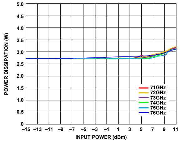
Figure 37. Power Dissipation vs. Input Power over Various Frequencies, I_{DD} = 700 mA, T_A = 85°C
