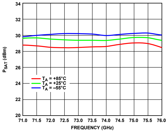
Figure 16. P_{SAT} vs. Frequency over Various Temperatures, I_{DD} = 800 mA
