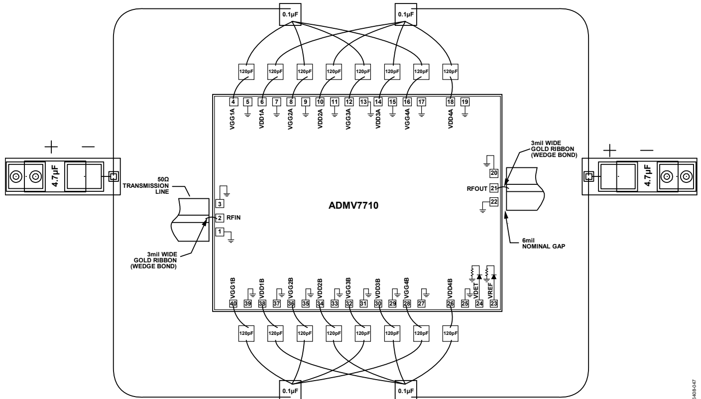
Figure 47. Assembly Diagram
