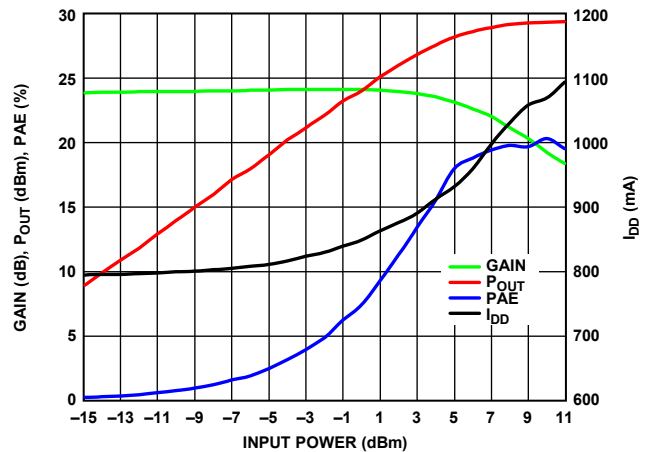
Figure 32. Gain, P_{OUT} , PAE, and I_{DD} vs. Input Power, RF = 73.5\text{ GHz} , I_{DD} = 800\text{ mA}
