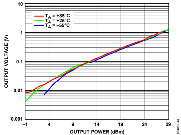
Figure 44. Detector Output Voltage ( V_{OUT} ) vs. Output Power over Various Temperatures, I_{DD} = 800\text{ mA} , R_F = 76\text{ GHz}
