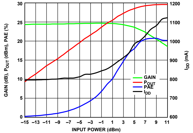
Figure 31. Gain, P_{OUT} , PAE, and I_{DD} vs. Input Power, RF = 71\text{ GHz} , I_{DD} = 800\text{ mA}
