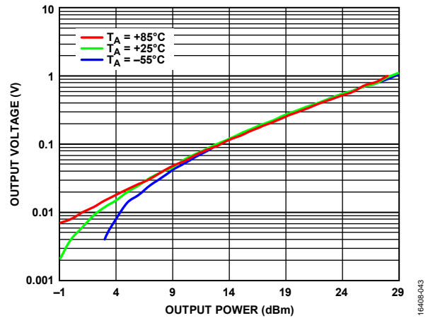
Figure 43. Detector Output Voltage ( V_{OUT} ) vs. Output Power over Various Temperatures, I_{DD} = 800\text{ mA} , R_F = 73.5\text{ GHz}
