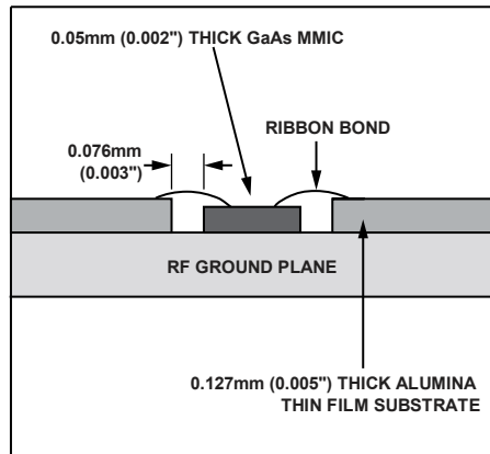
Figure 48. Routing RF Signals
