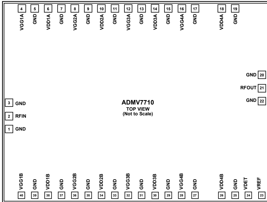
Figure 2. Pad Configuration
