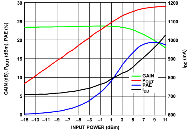
Figure 30. Gain, P_{OUT} , PAE, and I_{DD} vs. Input Power, RF = 76\text{ GHz} , I_{DD} = 700\text{ mA}
