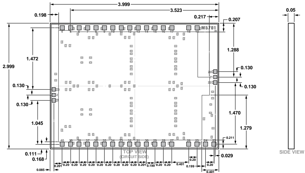
Figure 49. 40-Pad Bare Die [CHIP] (C-40-2) Dimensions shown in millimeters
