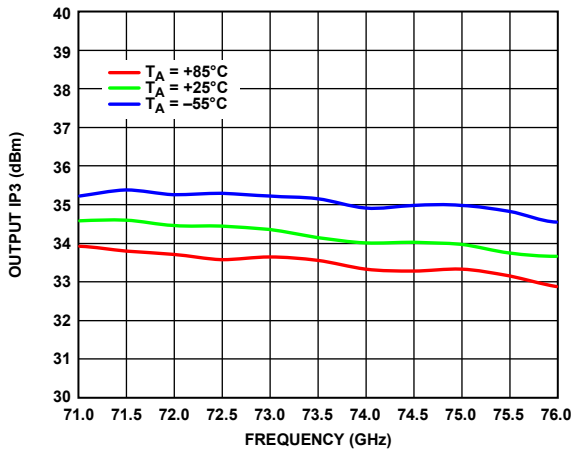
Figure 17. Output IP3 vs. Frequency over Various Temperatures, I_{DD} = 800 mA, P_{OUT} per Tone = 14 dBm
