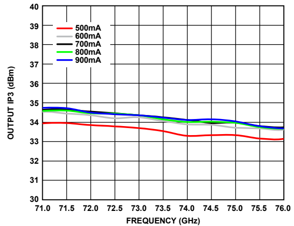
Figure 20. Output IP3 vs. Frequency over I_{DD} , P_{OUT} per Tone = 14 dBm
