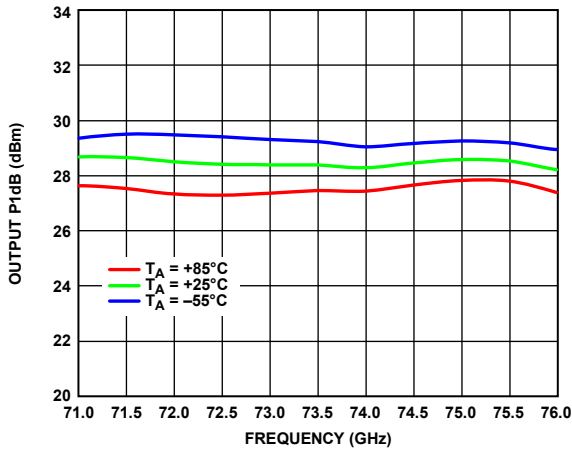
Figure 15. Output P1dB vs. Frequency over Various Temperatures, I_{DD} = 800 mA
