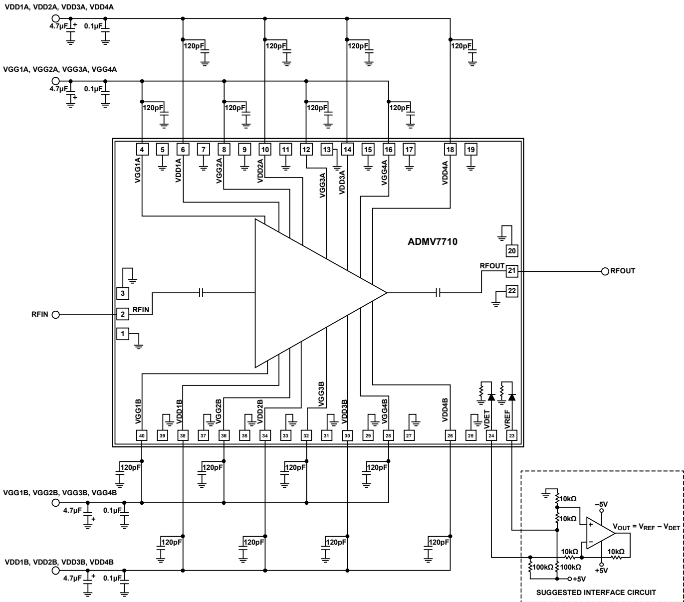
Figure 46. Typical Application Circuit
