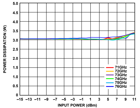
Figure 38. Power Dissipation vs. Input Power over Various Frequencies, I_{DD} = 800 mA, T_A = 85°C
