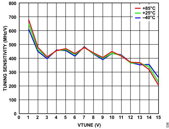
Figure 38. Tuning Sensitivity vs. VTUNE at Various Temperatures
