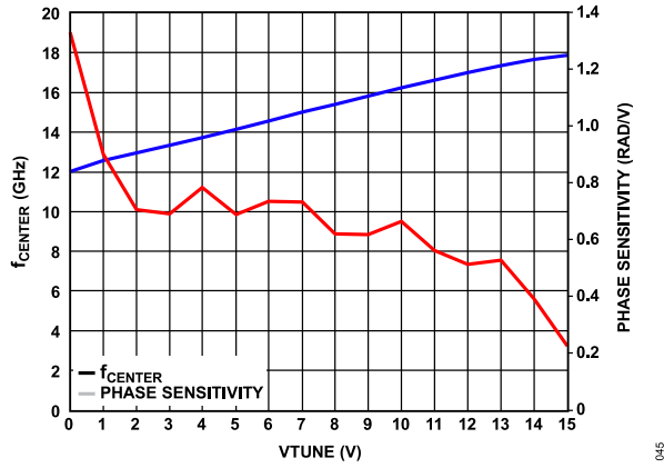
Figure 44. f CENTER and Phase Sensitivity vs. VTUNE, High Band
