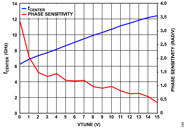
Figure 45. f CENTER and Phase Sensitivity vs. VTUNE, Low Band
