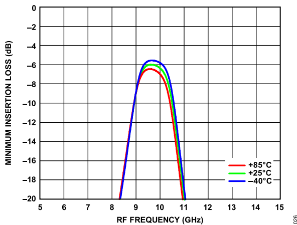
Figure 28. Minimum Insertion Loss vs. RF Frequency at Various Temperatures, VTUNE = 7 V
