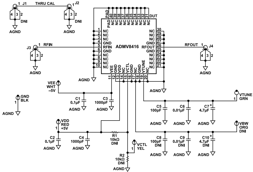
Figure 46. Typical Application Circuit
