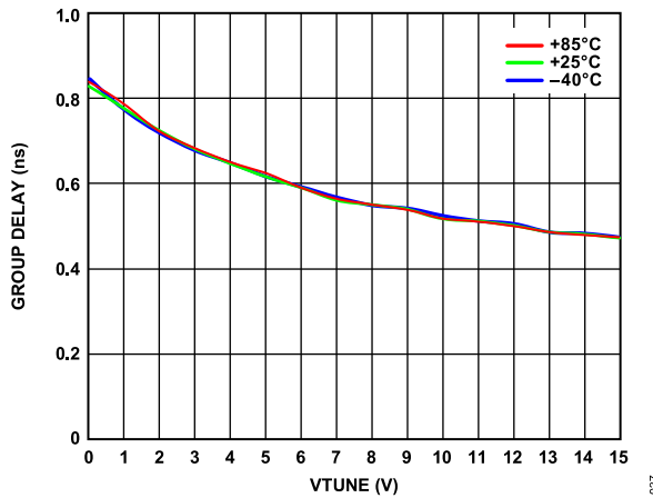
Figure 39. Group Delay vs. VTUNE at Various Temperatures
