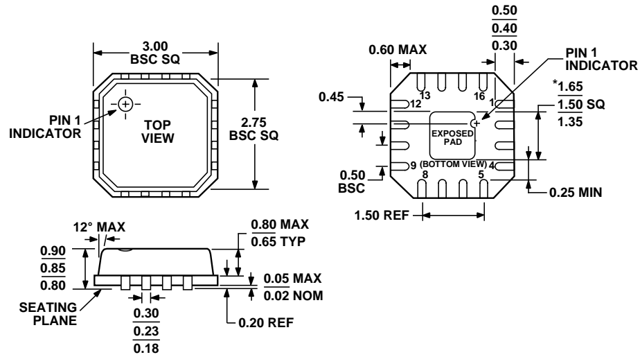
Figure 22. 16-Lead Lead Frame Chip Scale Package [VQ_LFCSP] 3 mm x 3 mm Body, Very Thin Quad (CP-16-3) Dimensions shown in millimeters
