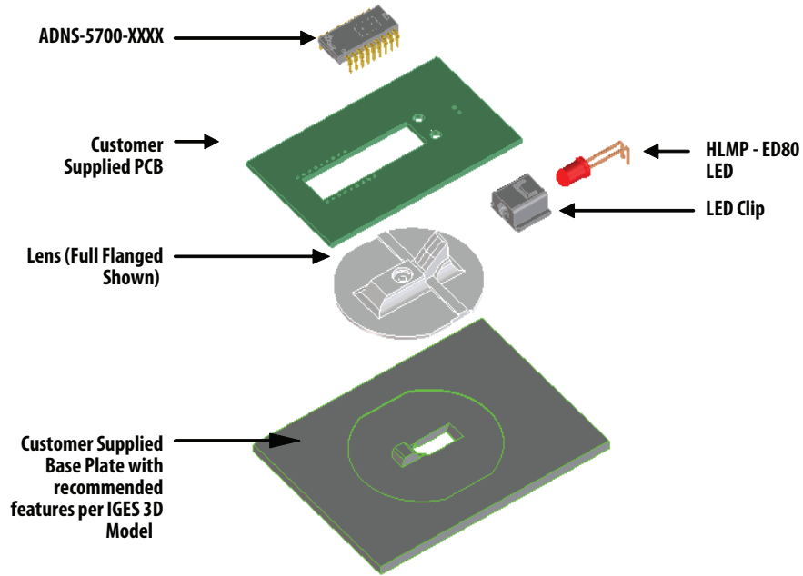
Figure 5. Exploded view drawing
