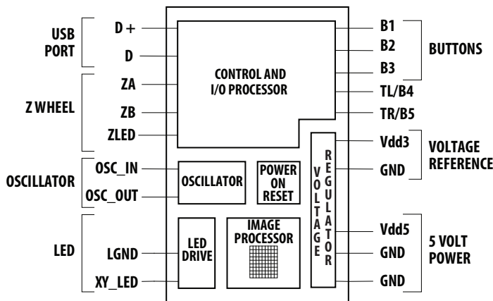
Figure 6. Block Diagram
