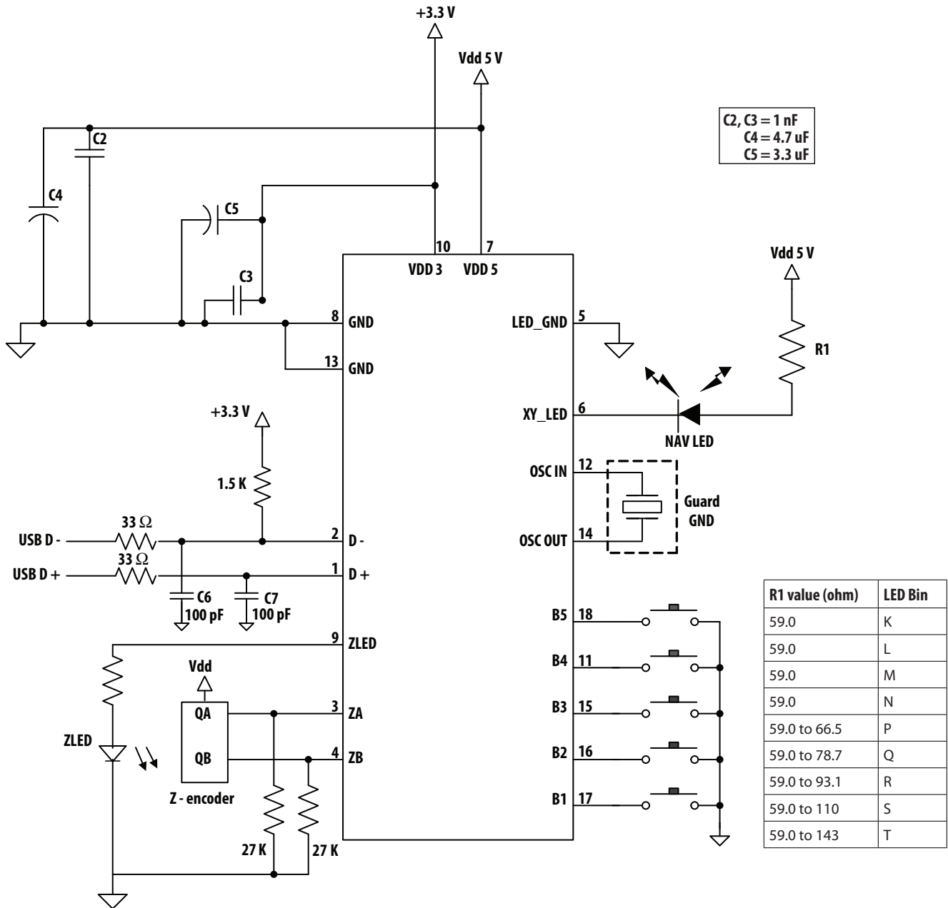
Figure 8c. Application Circuit ADNS-5700-HSPD and ADNS-5700-H5QD With 5 Button and Optical Z-Wheel
