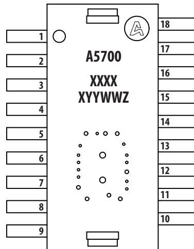
Figure 1a. Package pinout
