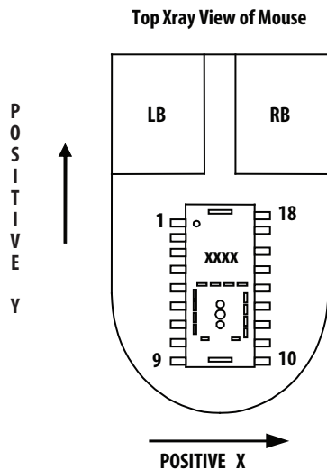
Figure 1b. Package pinout at 0°
