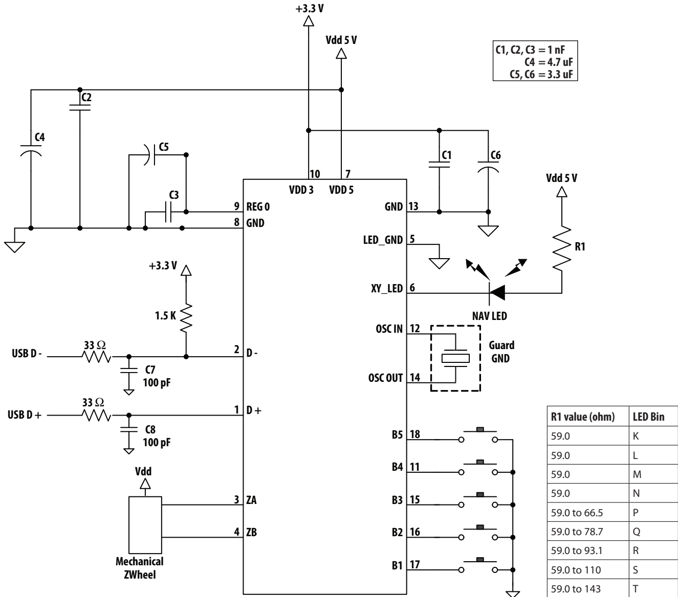
Figure 8d. Application Circuit with ADNS-5700-H5MD and ADNS-5700-H5ND with 5 Button and Mechanical Z-Wheel
