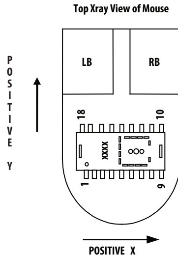
Figure 1c. Package pinout at 270°
