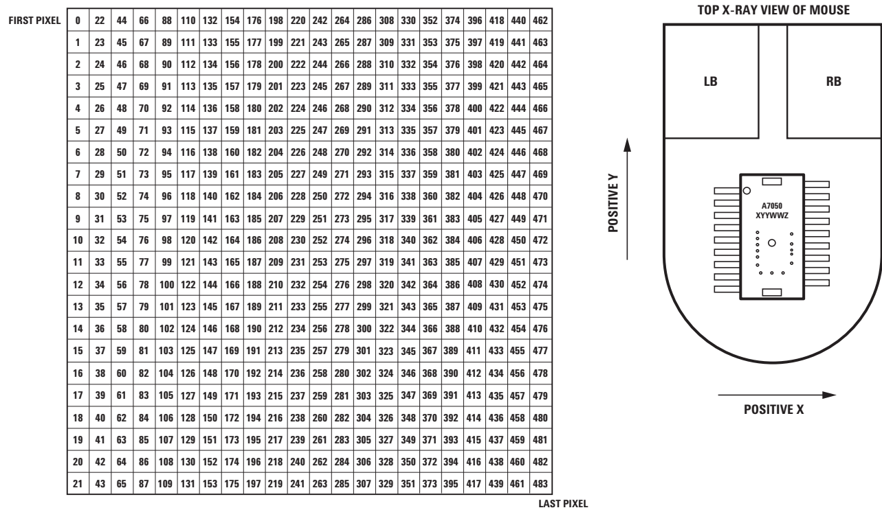
Figure 26. Pixel address map (looking through the ADNS-6130-001 or ADNS-6120 lens).
