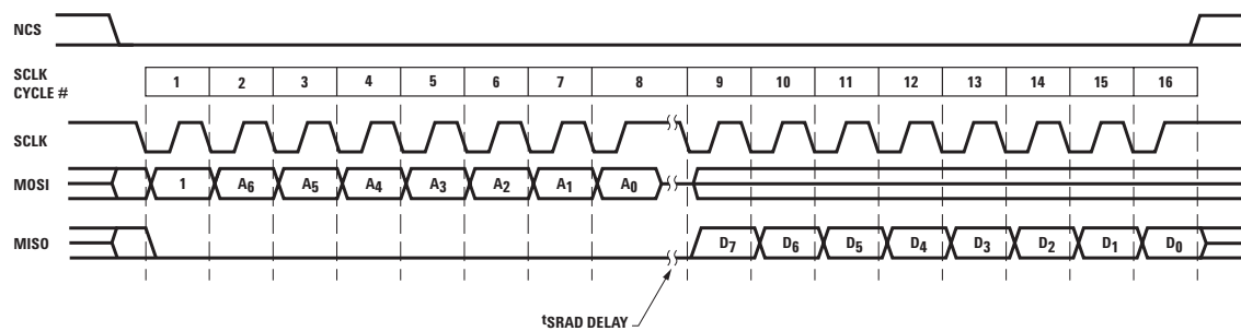
Figure 16. Read operation.
