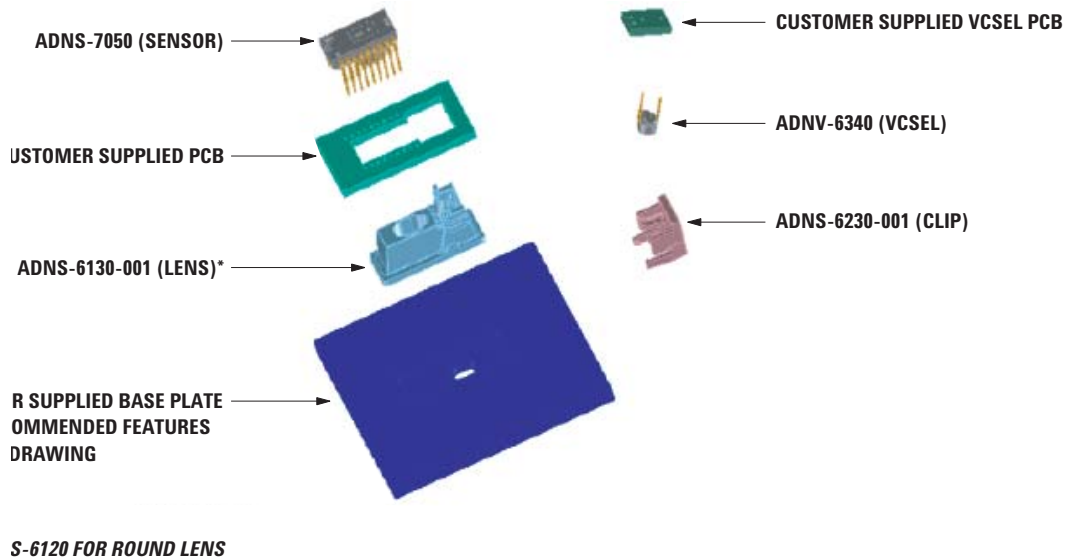
Figure 4. Exploded view drawing.
