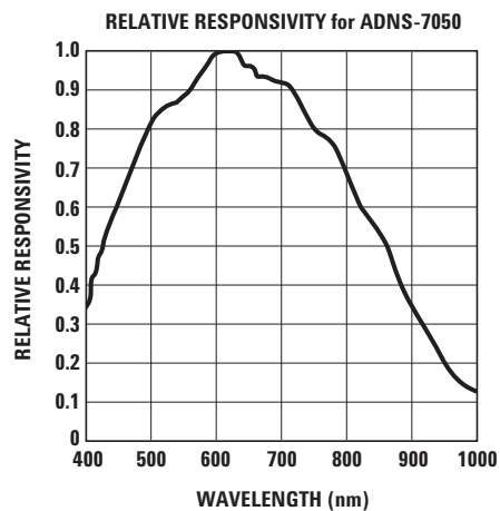
Figure 13. Wavelength responsivity.
