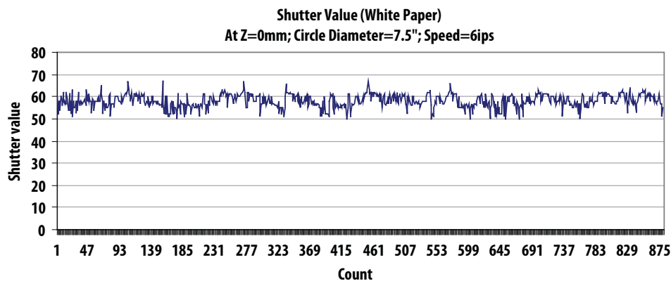
Figure 24. Shutter Values at 800cpi (White Paper)
