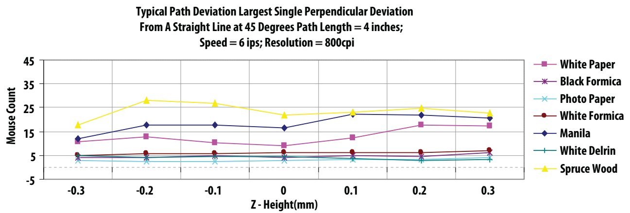
Figure 11. Average Error vs. Distance at 800dpi (mm)
