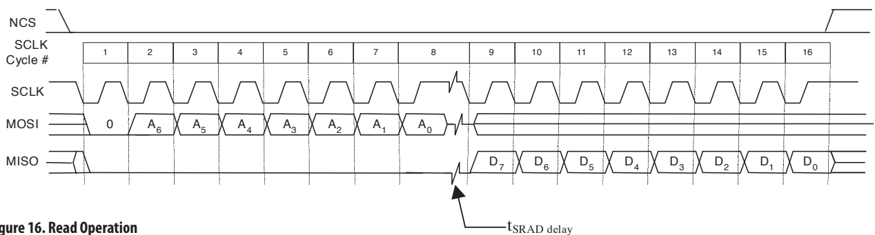
Figure 16. Read Operation
