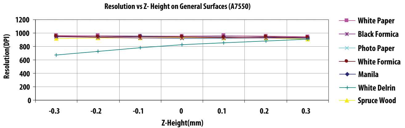
Figure 10. Mean Resolution vs. Z at 800dpi
