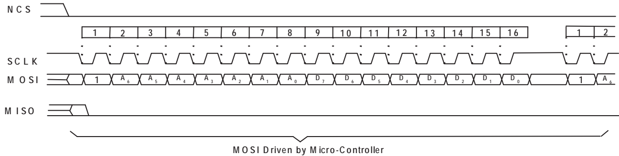
Figure 14. Write Operation
