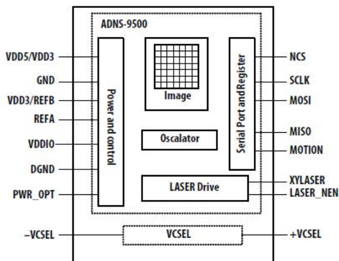
Figure 7. Block diagram of ADNS-9500
