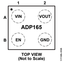
Figure 8. 4-Ball WLCSP Pin Configuration
