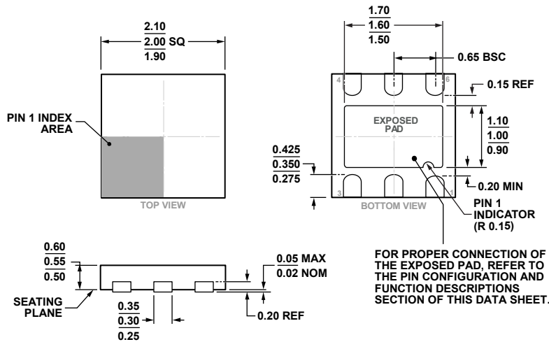
Figure 63. 6-Lead Lead Frame Chip Scale Package [LFCSPP_UD] 2.00 mm x 2.00 mm Body, Ultra Thin, Dual Lead (CP-6-3)
