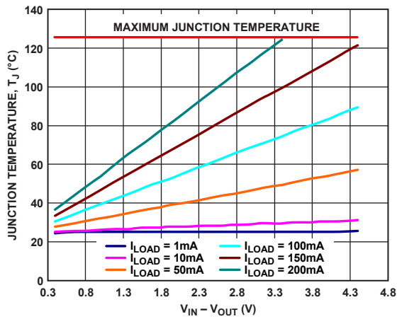
Figure 48. 100 mm 2 of PCB Copper, TSOT, T A = 25°C
