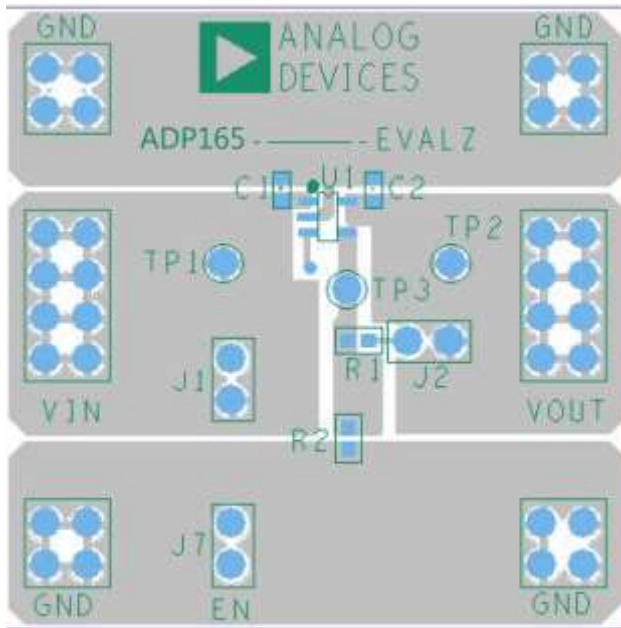
Figure 58. Example of 5-Lead TSOT PCB Layout
