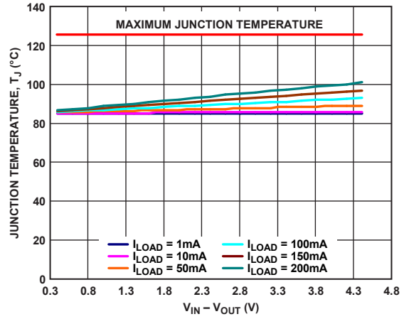
Figure 57. LFCSP, T A = 85°C
