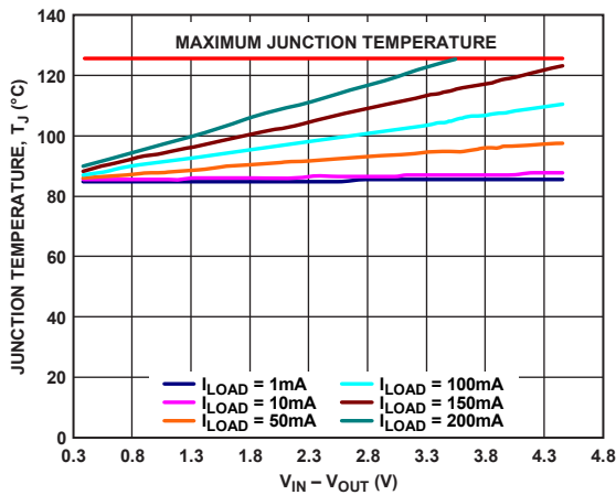
Figure 55. WLCSPP, T A = 85°C
