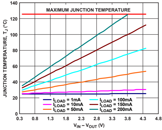
Figure 47. 500 mm 2 of PCB Copper, TSOT, T A = 25°C
