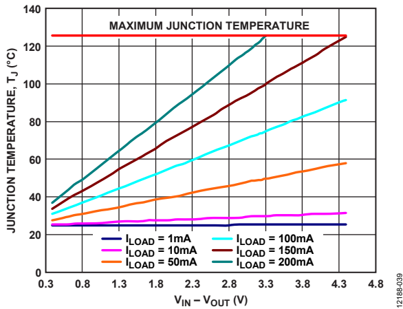
Figure 43. 500 mm 2 of PCB Copper, WLCSP, T_A = 25^\circ\text{C}
