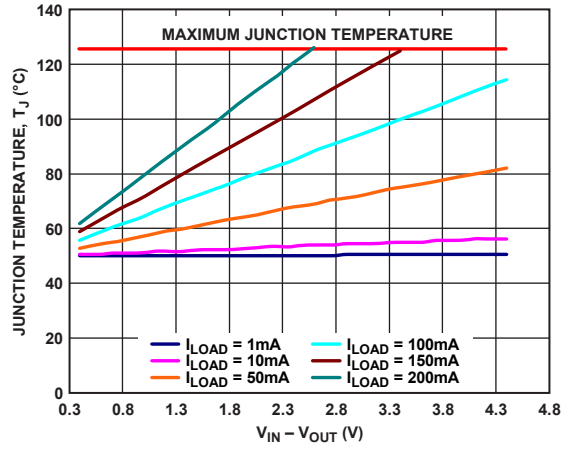
Figure 50. 100 mm 2 of PCB Copper, TSOT, T A = 50°C
