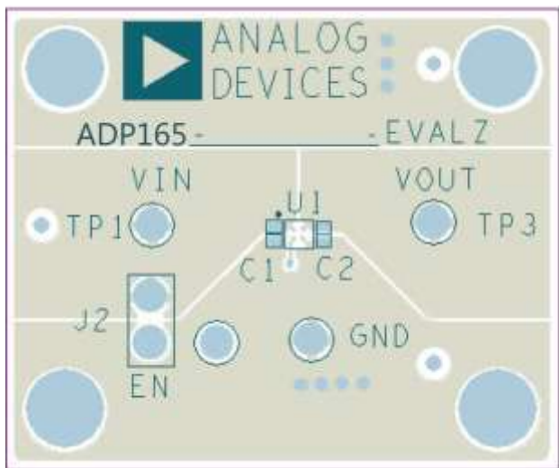
Figure 59. Example of 4-Ball WLCSP PCB Layout
