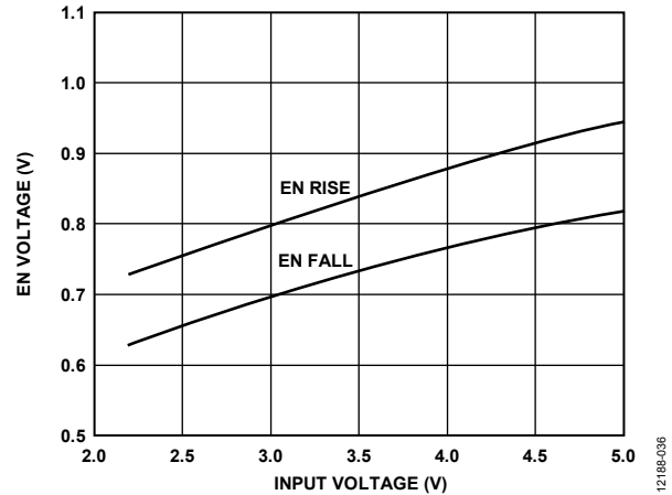
Figure 40. Typical EN Pin Thresholds vs. Input Voltage
