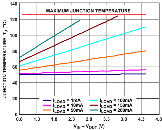
Figure 54. 100 mm 2 of PCB Copper, LFCSP, T A = 50°C
