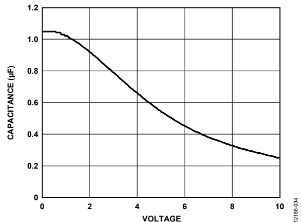
Figure 38. Capacitance vs. Voltage Characteristic
