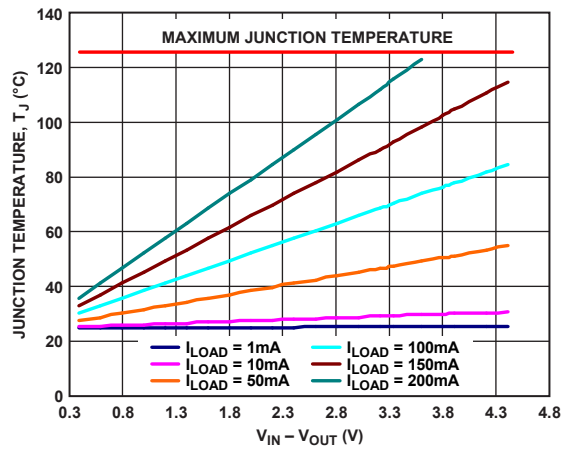
Figure 52. 100 mm 2 of PCB Copper, LFCSP, T A = 25°C
