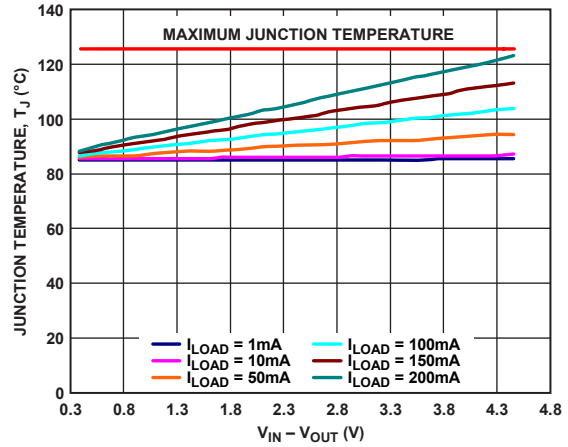
Figure 56. TSOT, T A = 85°C
