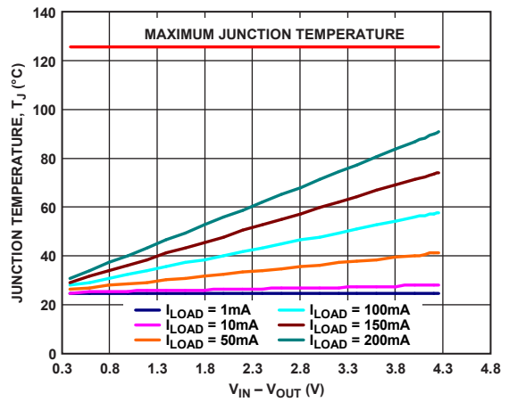
Figure 51. 500 mm 2 of PCB Copper, LFCSP, T A = 25°C
