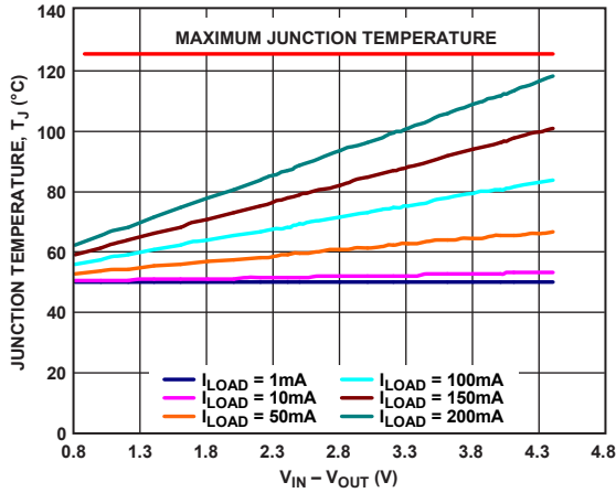
Figure 53. 500 mm 2 of PCB Copper, LFCSP, T A = 50°C
