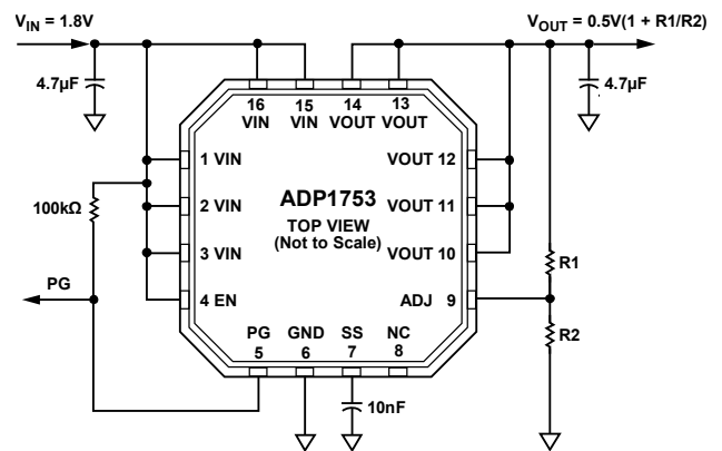
Figure 2. ADP1753 with Adjustable Output Voltage, 0.75 V to 3.0 V
