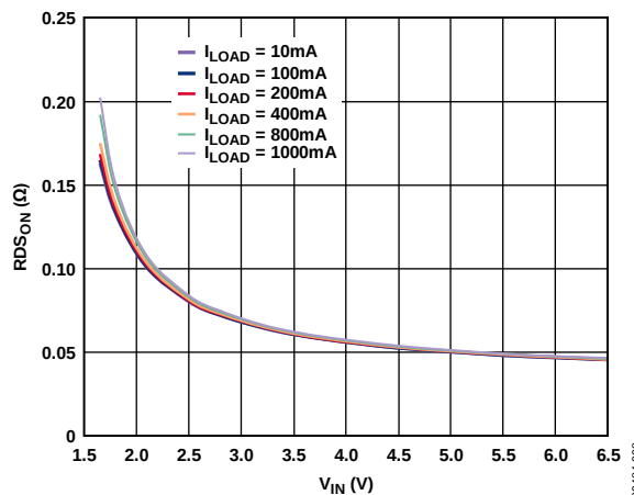
Figure 8. R_{DS(on)} vs. Input Voltage ( V_{IN} ), WLCSP
