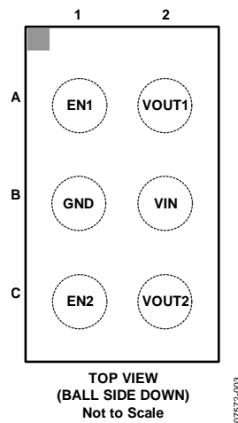
Figure 3. Pin Configuration
