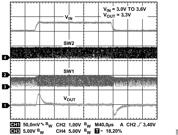
Figure 16. Line Transient, PWM Mode ( V_{IN} = 3.0\text{ V to }3.6\text{ V} , V_{OUT} = 3.3\text{ V} )
