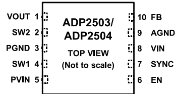
Figure 2. Pin Configuration
