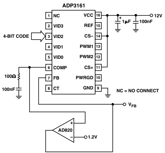
TPC 1. Closed-Loop Output Voltage Accuracy Test Circuit
