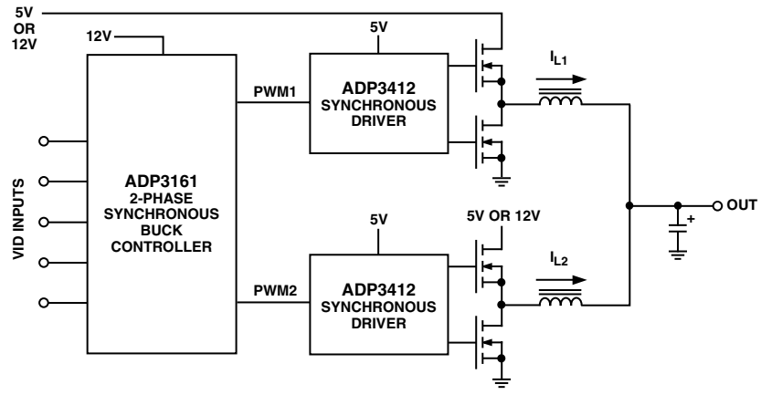
TPC 5. 2-Phase CPU Supply System Level Block Diagram
