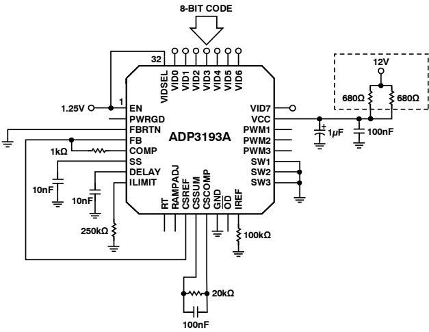
Figure 4. Closed-Loop Output Voltage Accuracy
