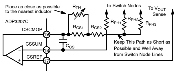
Figure 29. Temperature Compensation Circuit Values
