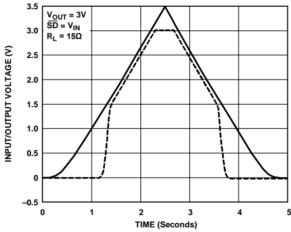
Figure 11. Power-Up/Power-Down
