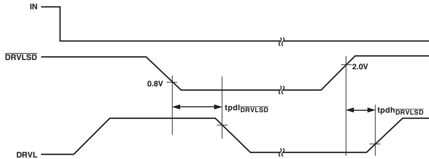
Figure 3. \overline{DRVLS} Propagation Delay
