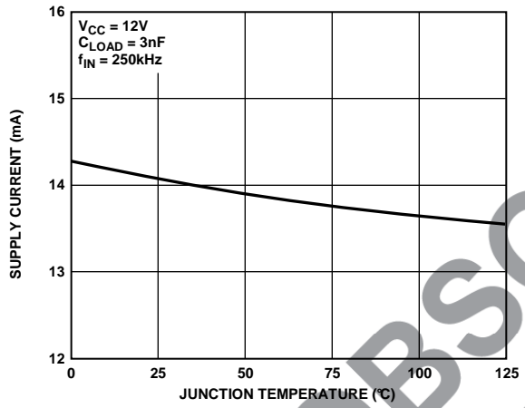
Figure 12. Supply Current vs. Junction Temperature
