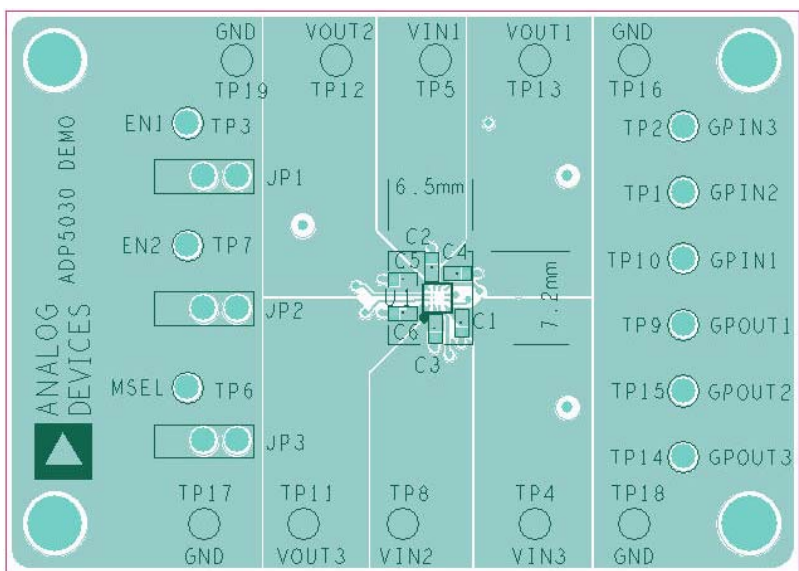
Figure 50. Example of PCB Layout, Top Side
