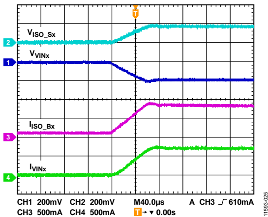
Figure 22. Input Current-Limit Transition from 100 mA to 900 mA, I_{ISO\_Sx} Load = 66 \Omega , Charging = 750 mA
