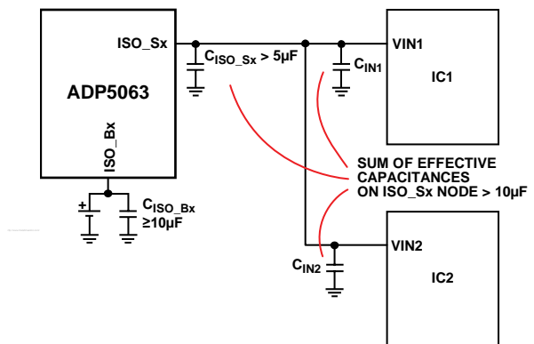
Figure 36. Splitting ISO_Sx Capacitance
