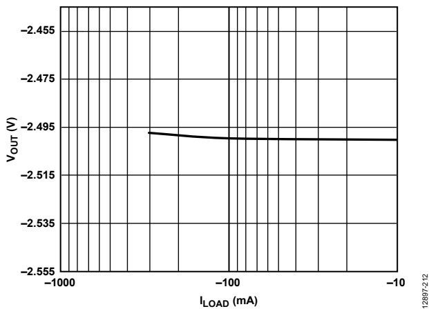
Figure 12. Output Voltage ( V_{OUT} ) vs. Load Current ( I_{LOAD} ), V_{OUT} = -2.5 V
