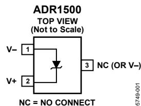
Figure 1. 3-Lead SC70 (KS Suffix)
