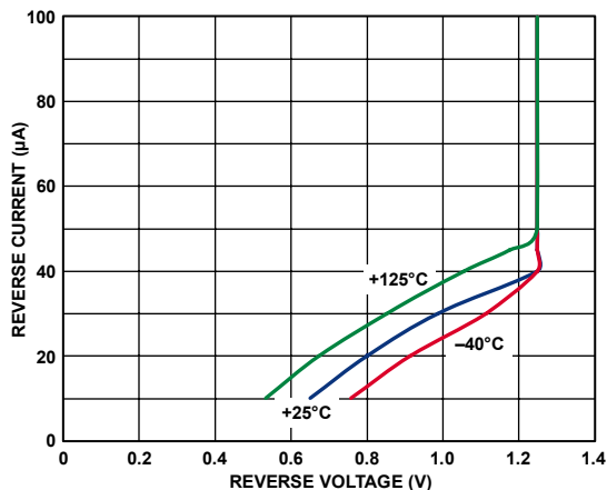
Figure 7. Reverse Current vs. Reverse Voltage
