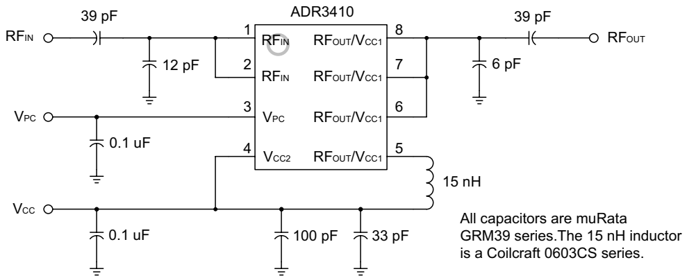
Figure 3: 869 - 894 MHz Application Circuit (50 Ω Terminations)
