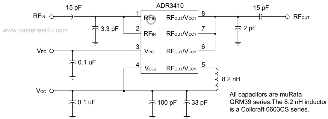
Figure 4: 2110 - 2170 MHz Application Circuit (50 \Omega Terminations)
