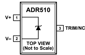
Figure 1. 3-Lead SOT-23-3
