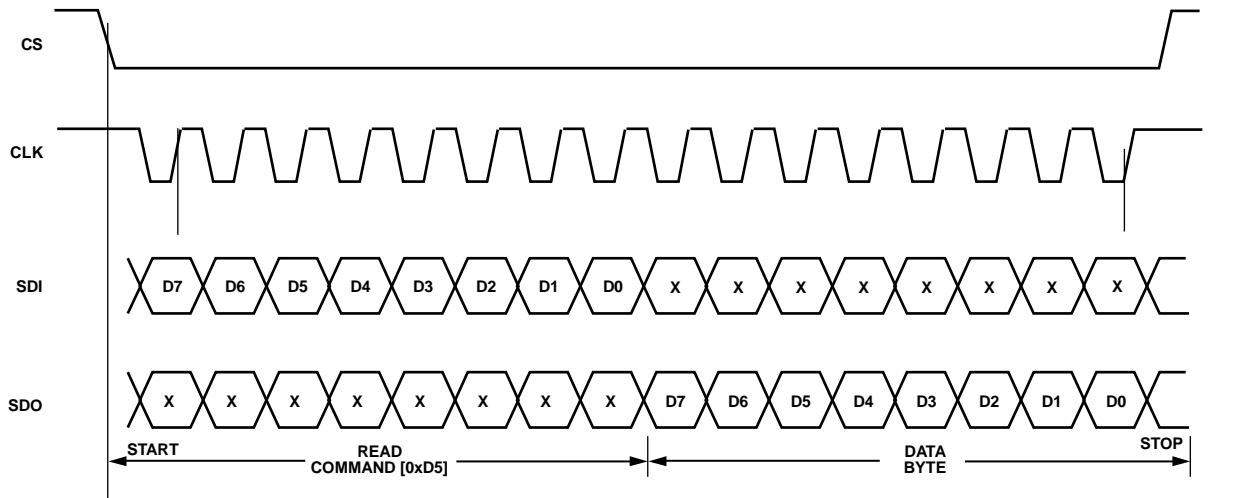
Figure 69. SPI Byte Read Example
