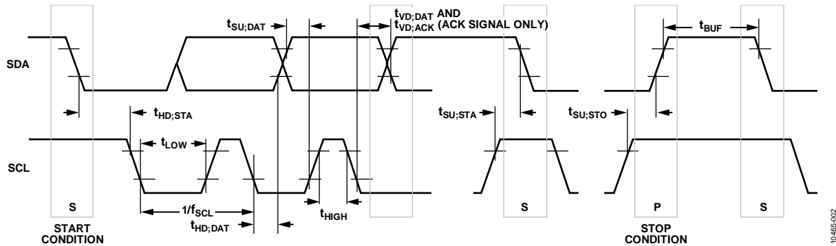
Figure 2. I 2 C Port Timing Diagram
