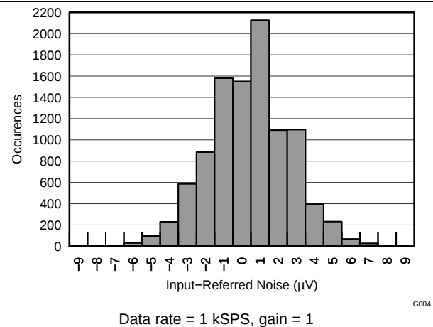
Figure 4. Noise Histogram
