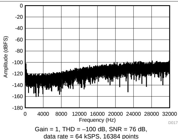
Figure 12. FFT Plot
