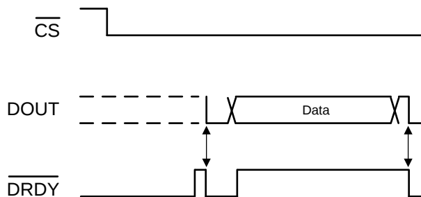
Figure 36. Using DOUT as \overline{\text{DRDY}}
