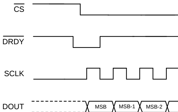
Figure 37. \overline{\text{DRDY}} Behavior with Data Retrieval
