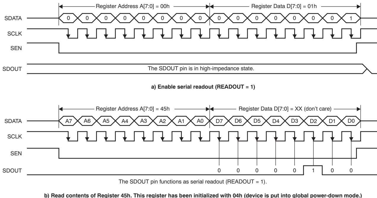
Figure 48. Serial Readout Timing Diagram
