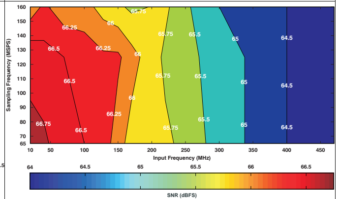
Figure 38. Signal-To-Noise Ratio (6dB Gain)
