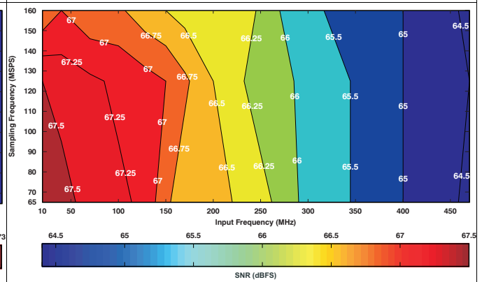
Figure 36. Signal-To-Noise Ratio (6dB Gain)
