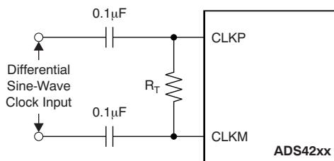
Figure 50. Differential Sine-Wave Clock Driving Circuit
