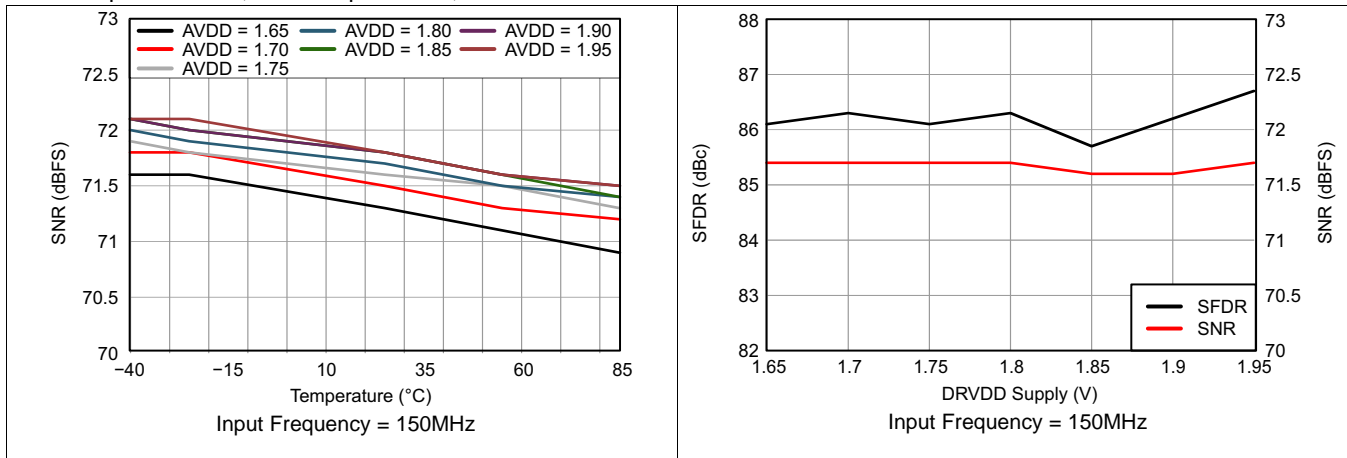
Figure 22. Performance vs DRVDD Supply Voltage
