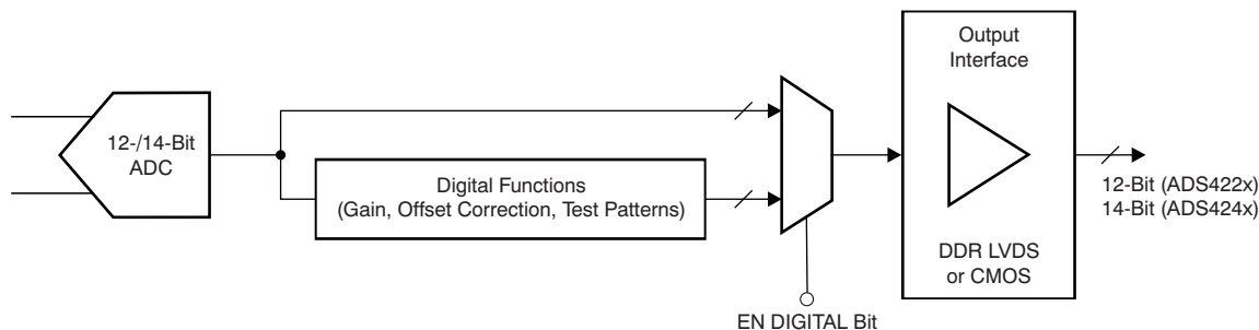
Figure 39. Digital Processing Block
