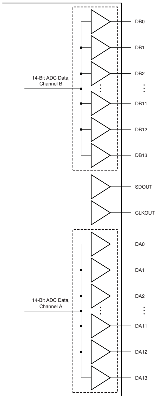
Figure 44. CMOS Outputs
