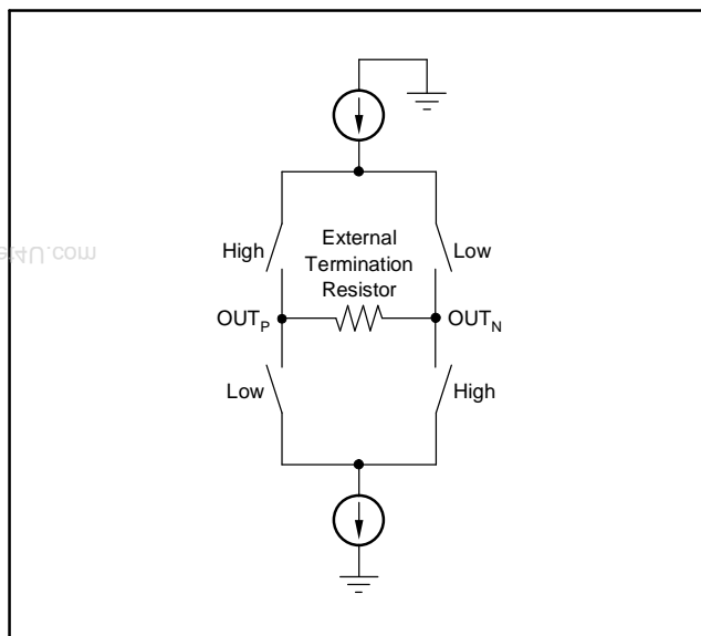
Figure 37. LVDS Buffer
