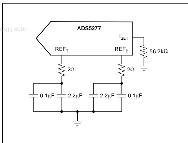
Figure 36. Internal Reference
