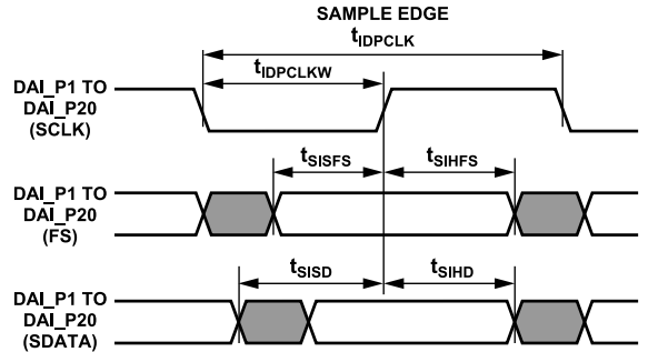
Figure 17. IDP Main Timing
