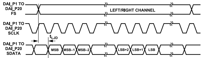
Figure 24. Left-Justified Mode
