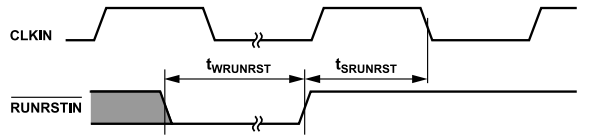
Figure 5. Running Reset
