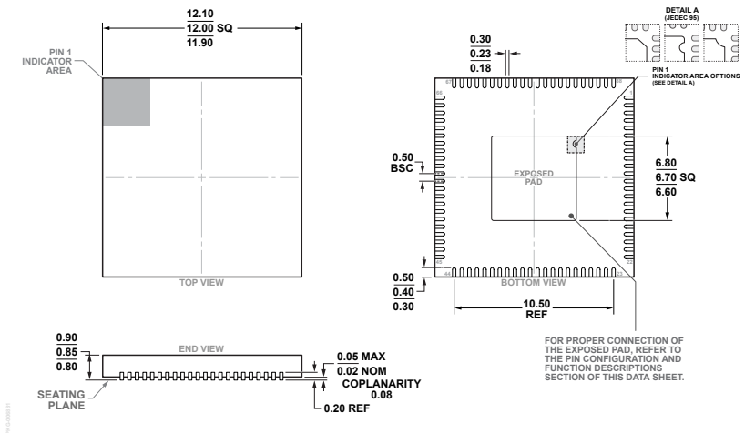
Figure 39. 88-Lead Lead Frame Chip Scale Package [LFCSP] 12 x 12 mm Body and 0.85 mm Package Height (CP-88-11) Dimensions shown in millimeters
