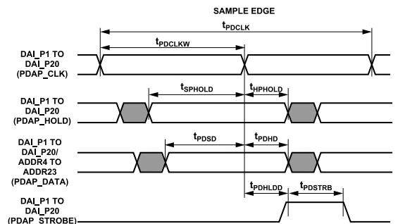
Figure 18. PDAP Timing
