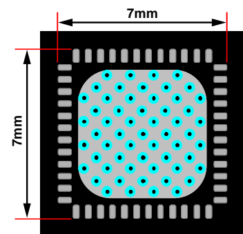
LAND PATTERN-TOP LAYER
