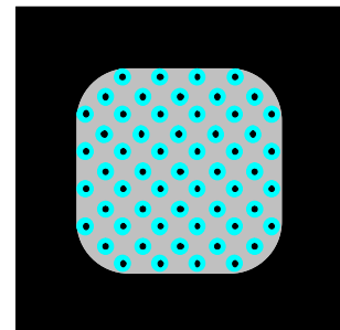
LAND PATTERN-BOTTOM LAYER
