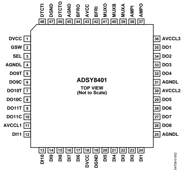
Figure 2. Pin Configuration
