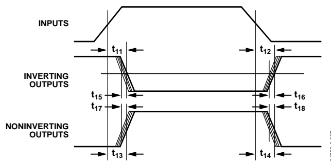
Figure 7. Inverting and Complementary Level Shifter Timing
