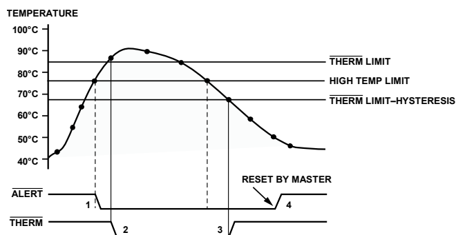
Figure 82. \overline{\text{THERM}} Behavior
