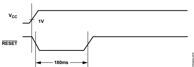
Figure 84. Operation of \overline{\text{RESET}} Output on Power-Up
