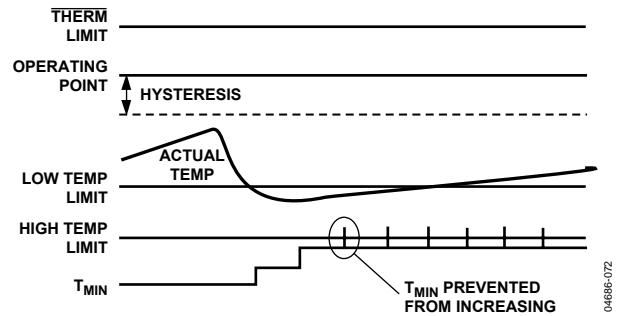
Figure 70. T_{MIN} Adjustments Limited by the High Temperature Limit
