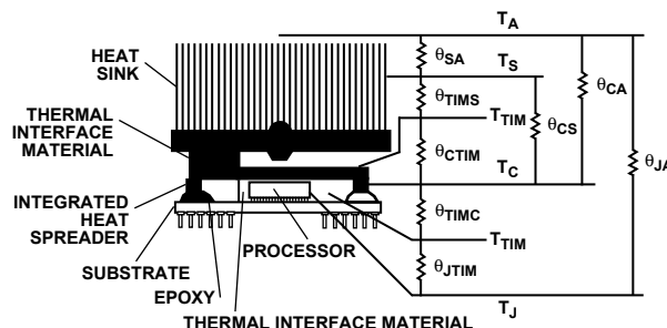
Figure 62. Thermal Model
