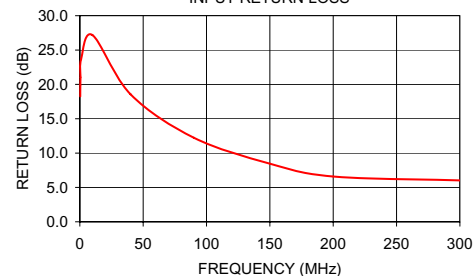
ADTT1-1 INPUT RETURN LOSS
