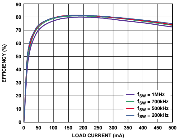
Figure 6. Typical Efficiency at Various Switching Frequencies with 1:2 Halo Transformer (TGSAD-560V8LF), 5 V Input to 5 V Output
