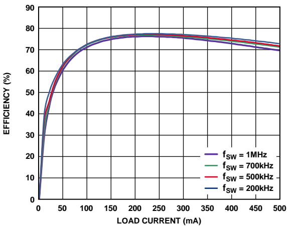
Figure 5. Typical Efficiency at Various Switching Frequencies with 1:2 Coilcraft Transformer (CR7983-CL), 5 V Input to 5 V Output
