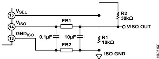
Figure 31. V_{\text{ISO}} Bias and Bypass Components
