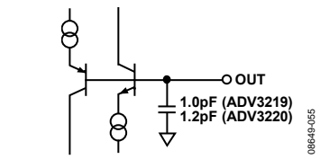
Figure 53. ADV3219/ADV3220 Disabled Output
