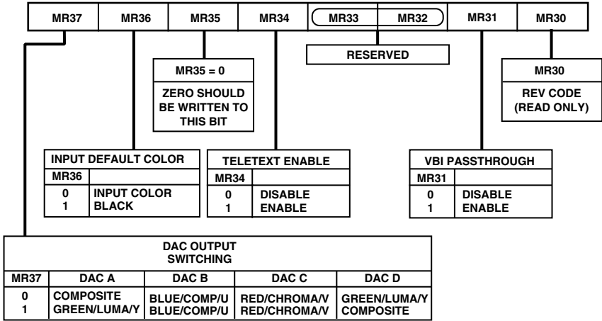
Figure 42. Mode Register 3
