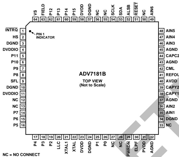
Figure 4. 64-Lead LFCSP/LQFP Pin Configuration
