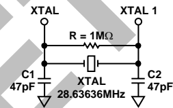
Figure 43. Crystal Circuit
