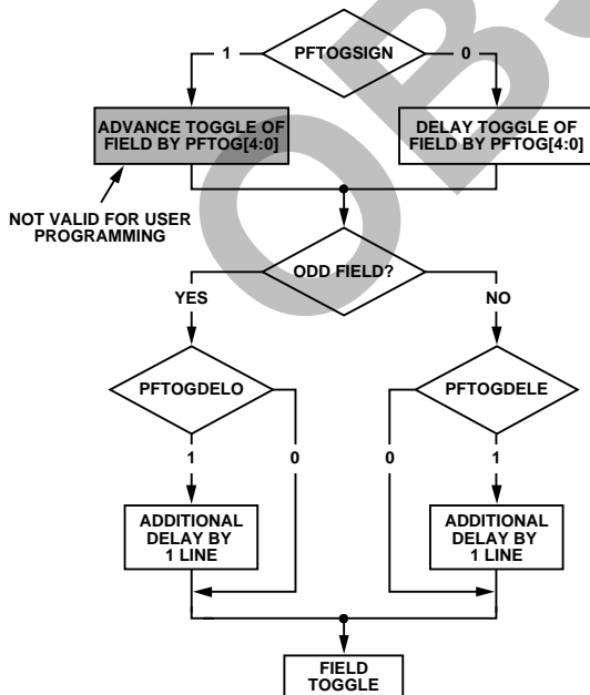
Figure 29. PAL F Toggle
