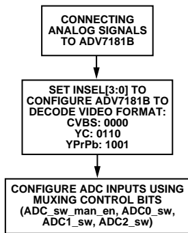
Figure 6. Input Muxing Overview
