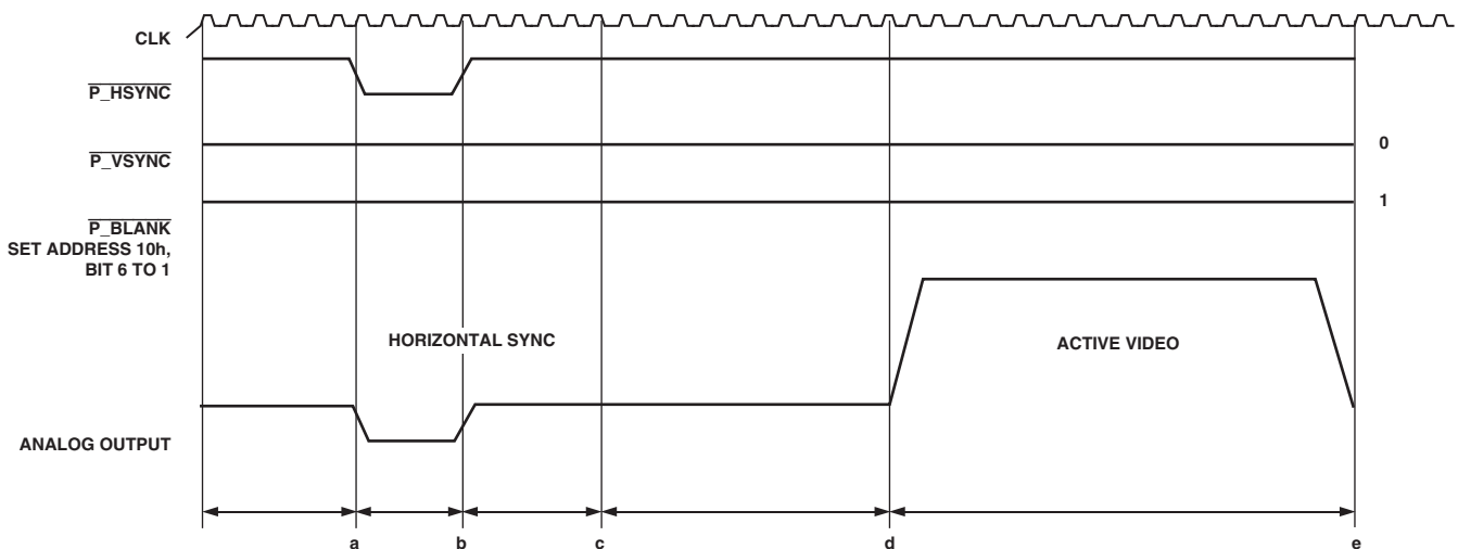
Figure 29b. Async Timing Mode—Programming Input Control Signals for Bilevel Sync Signal
