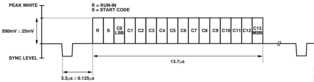
Figure 92. PS 625p CGMS-A Waveform (Line 43)
