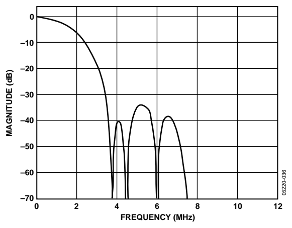
Figure 36. Luma QCIF Low-Pass Filter
