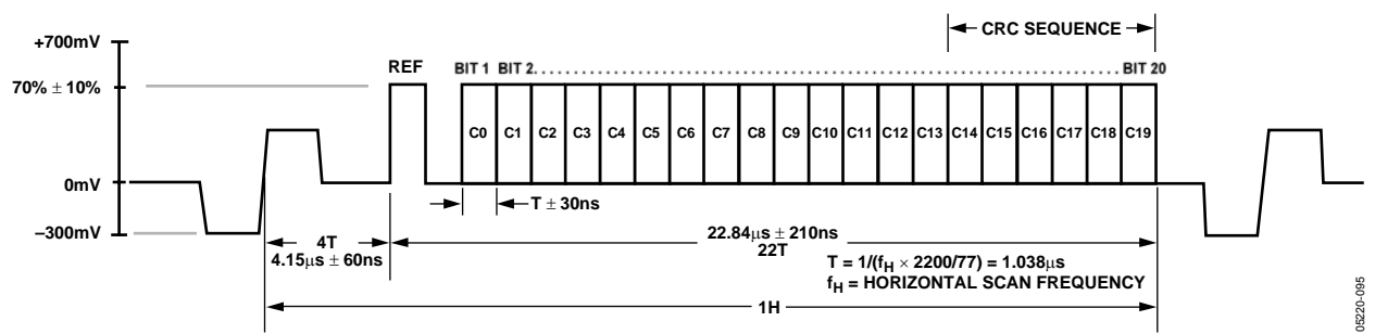
Figure 95. HDTV 1080i CGMS Waveform
