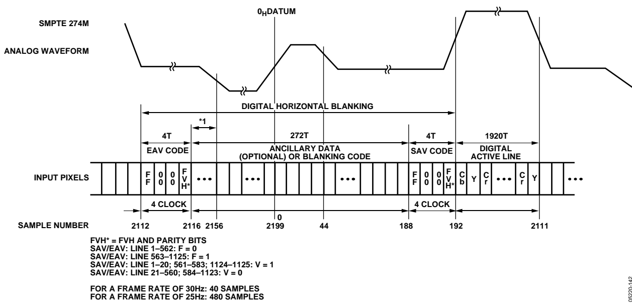
Figure 142. EAV/SAV Input Data Timing Diagram (SMPTE 274M)
