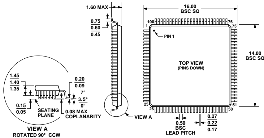
Figure 9. 100-Lead Low Profile Quad Flat Package [LQFP] (ST-100)
