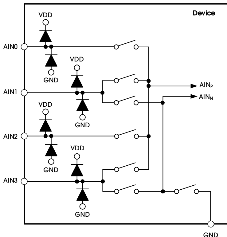
Figure 17. Input Multiplexer
