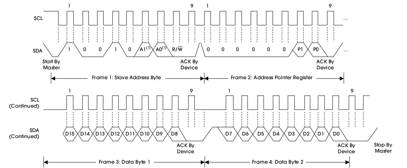
Figure 23. Timing Diagram for Writing to ADX111(Q)
